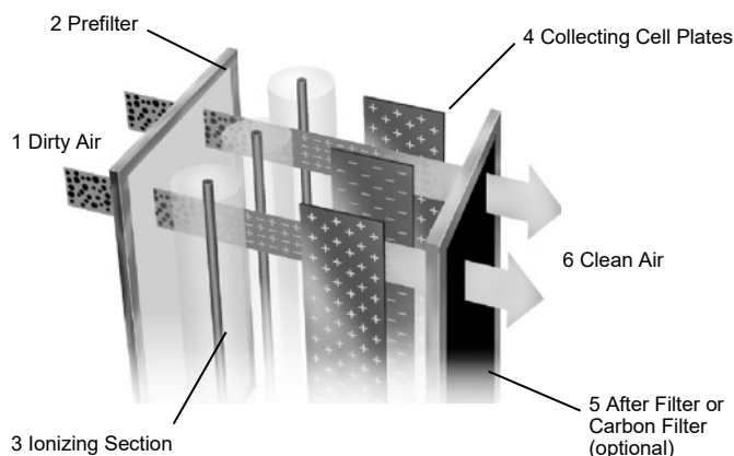
Electrostatic Precipitation
